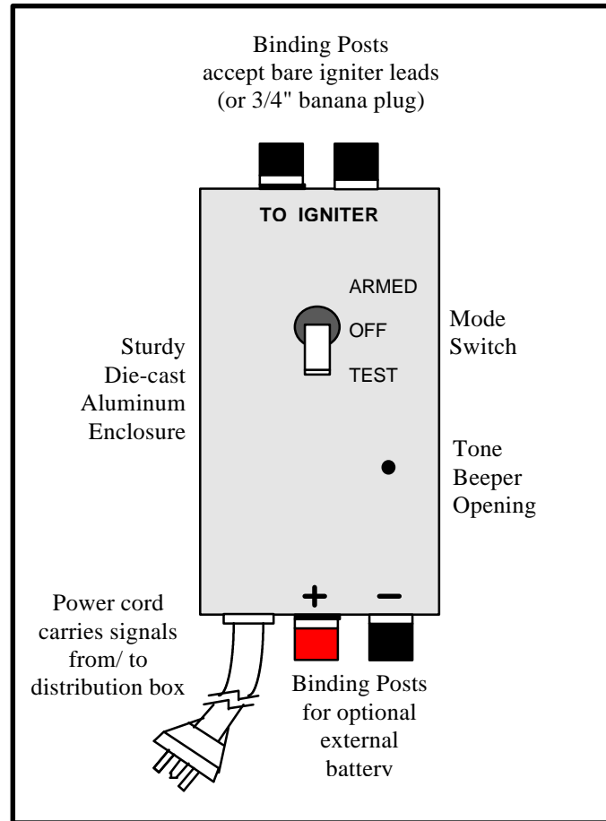
Pad Box Front View
