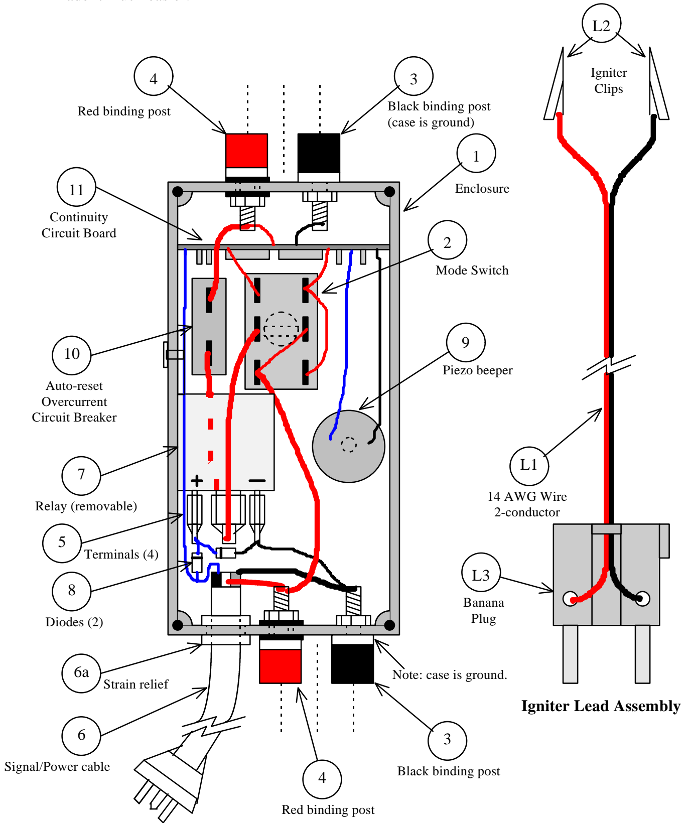
Pad Box Assembly (actual size)
