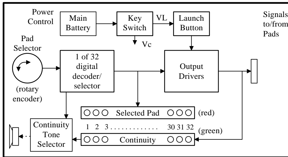
Main Control Console Block Diagram
