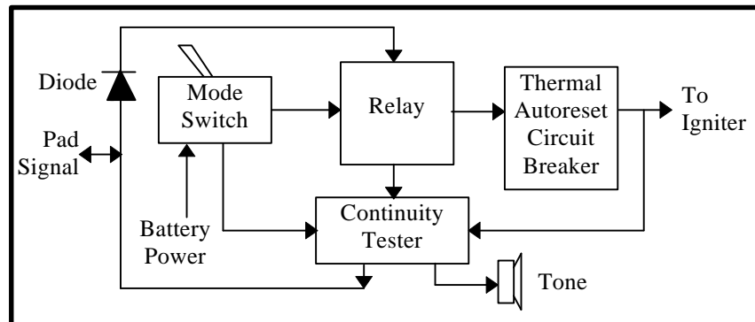
Pad Control Box Basic Components
